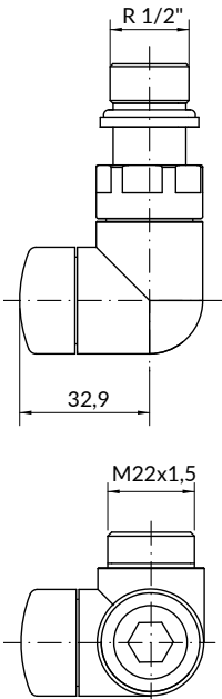
3-axis lockshield valve
