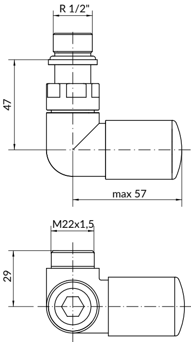
3-axis regulating valve
