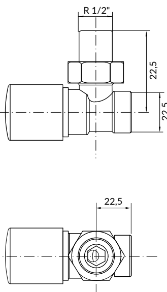
Shut-off valve
