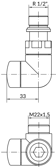
3-axis lockshield valve
