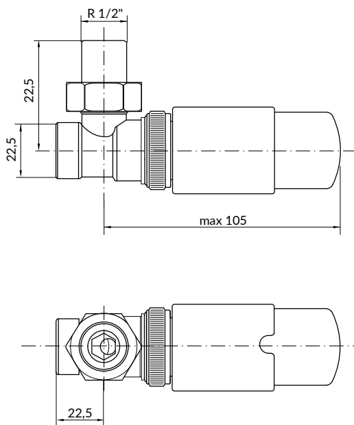
Thermostatic valve
