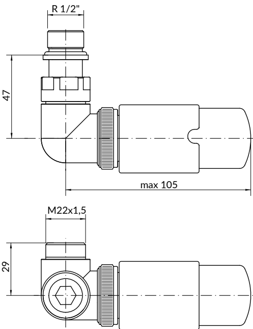
3-axis thermostatic valve
